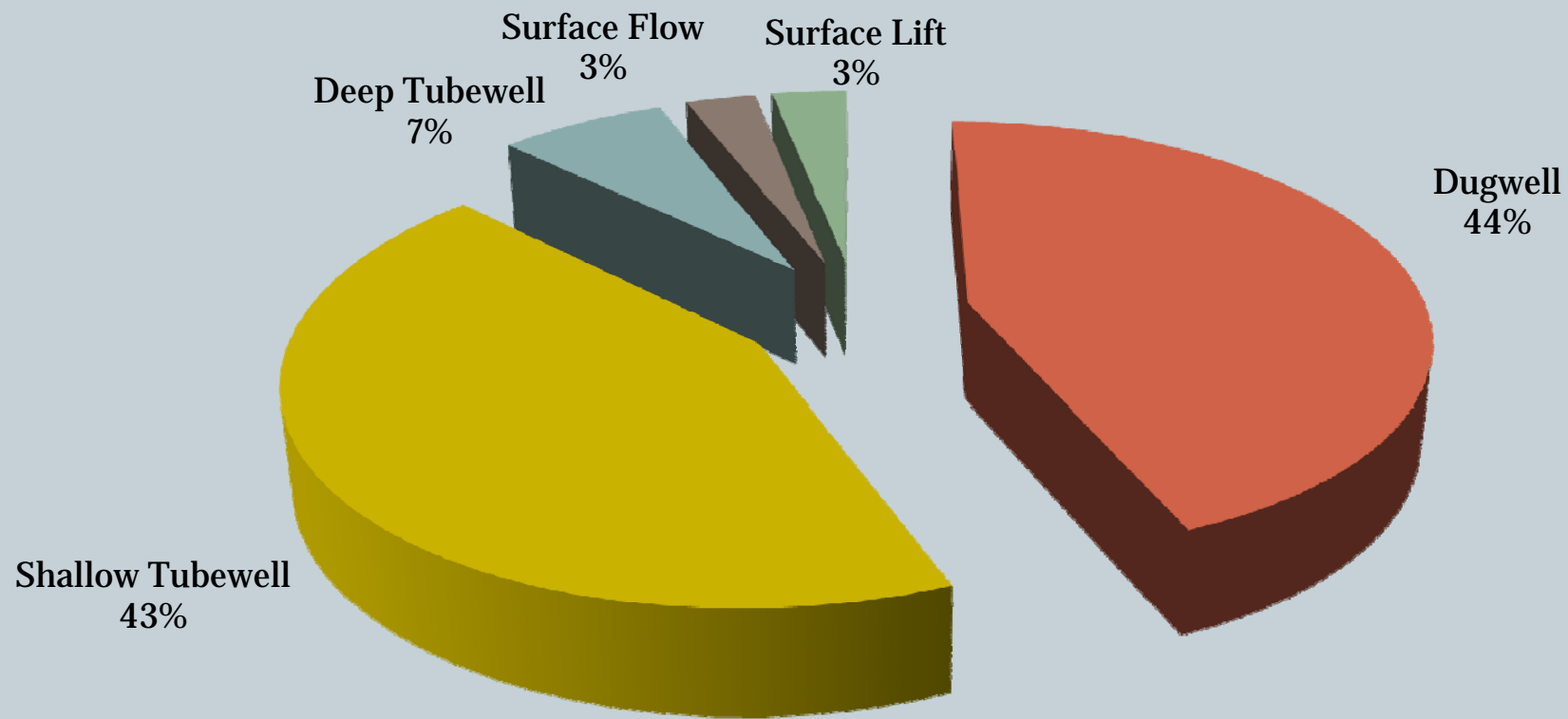
Share of MI Schemes by type
